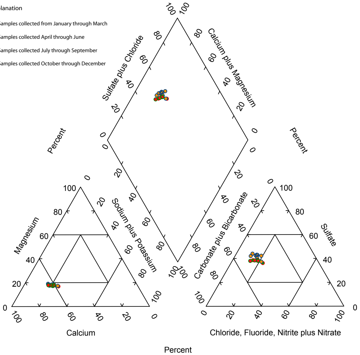
Figure 3. Trilinear plot for Roaring Fork River at Glenwood Springs (site 24).
