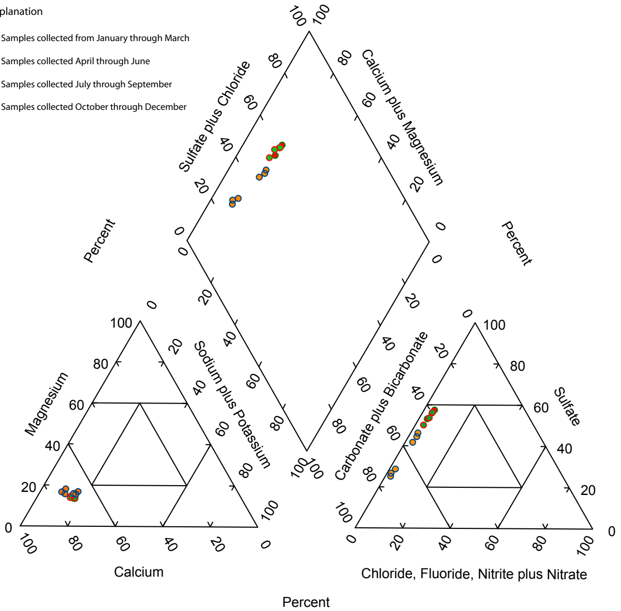
Figure 4. Trilinear plot for Crystal River above Avalanche Creek near Redstone (site 42).
