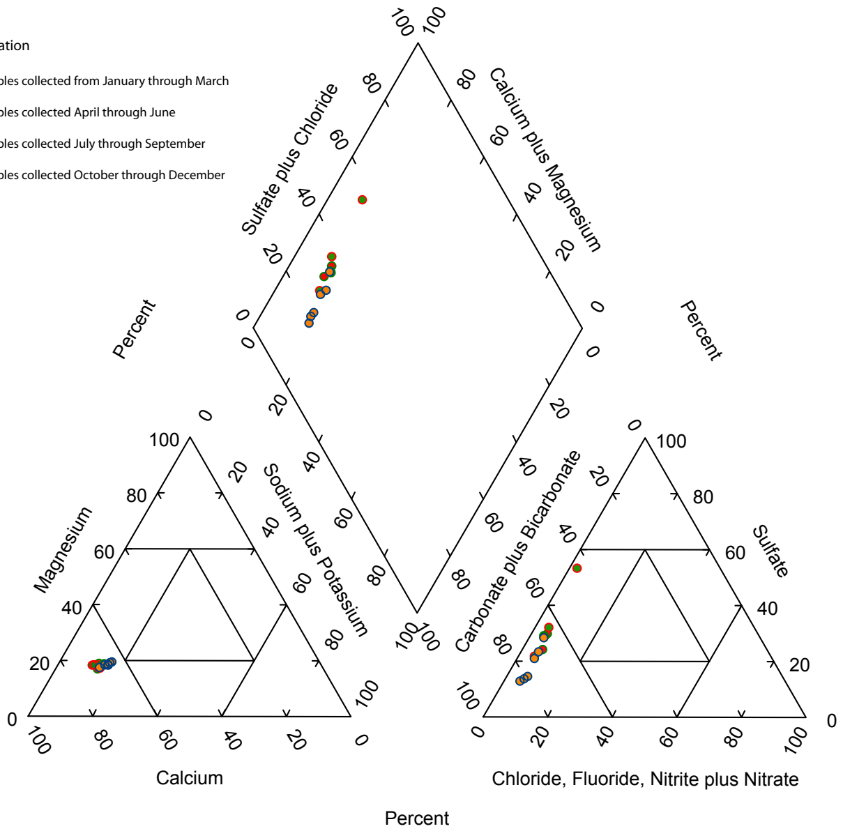
Figure 1. Trilinear plot for Roaring Fork River above Difficult Creek near Aspen (site 2).
