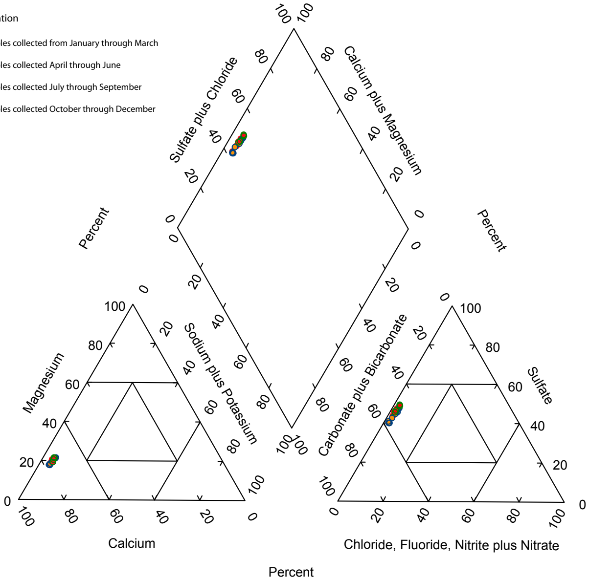
Figure 2. Roaring Fork River near Emma trilinear plot.
