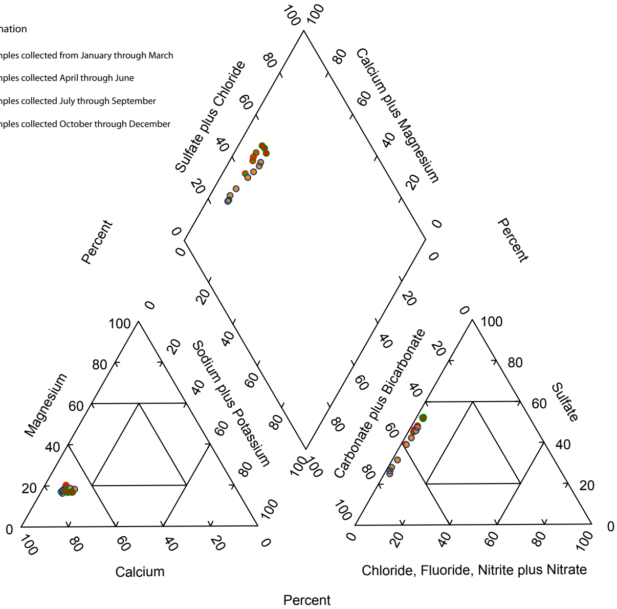
Figure 5. Trilinear plot for Crystal River below Carbondale (site 46).
